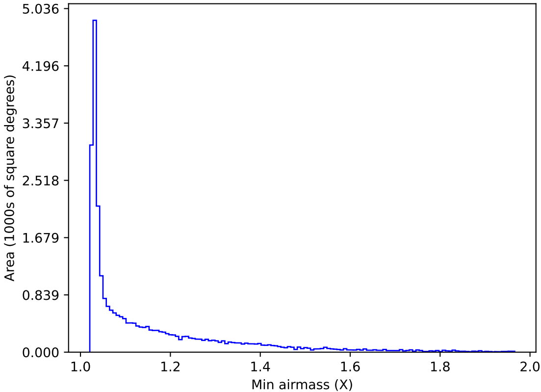
ddf_acor_sf10_lsf20_lsr20_v3.4_10yrs Yr 1 all bands: Min airmass
