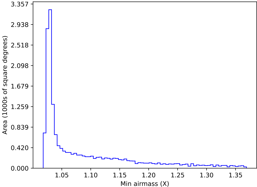
ddf_acor_sf10_lsf20_lsr20_v3.4_10yrs WFD z band: Min airmass
