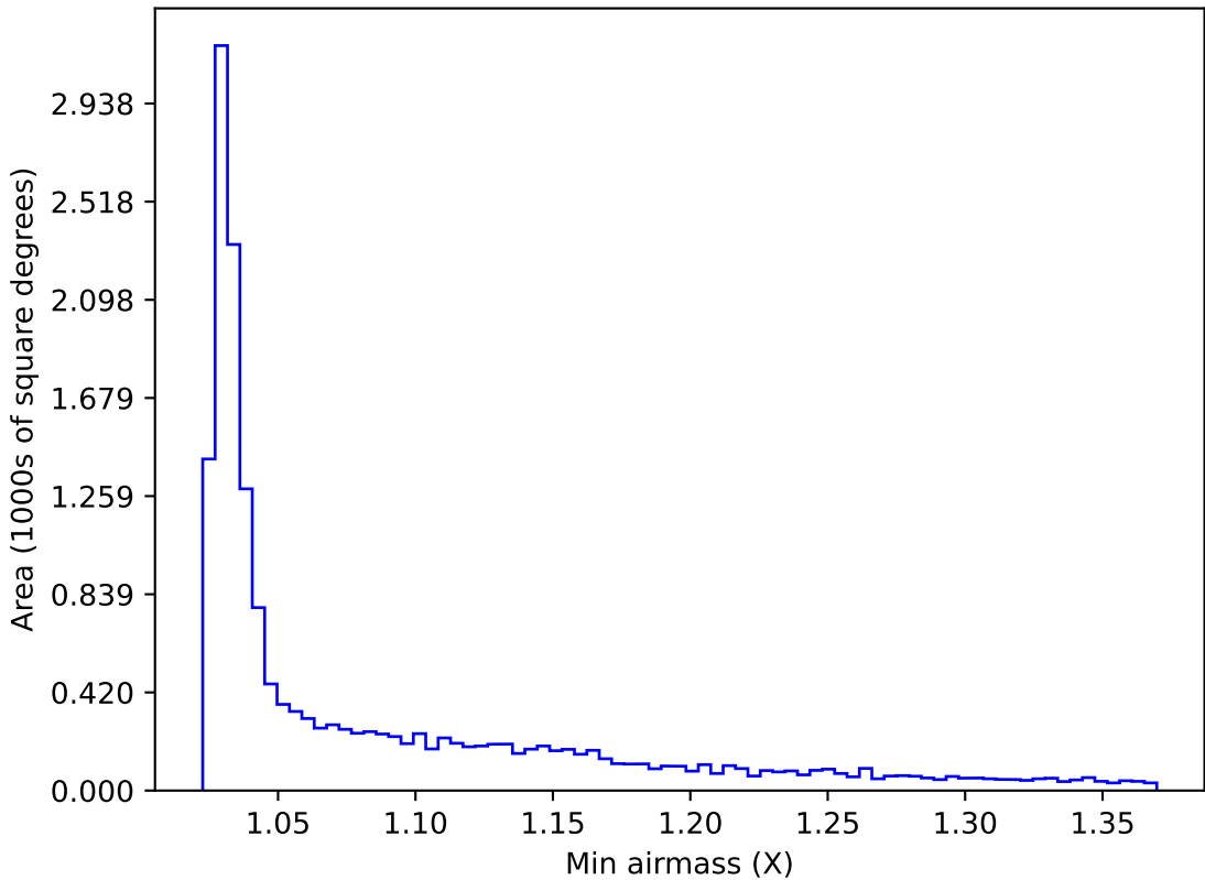
ddf_acor_sf10_lsf20_lsr20_v3.4_10yrs WFD y band: Min airmass
