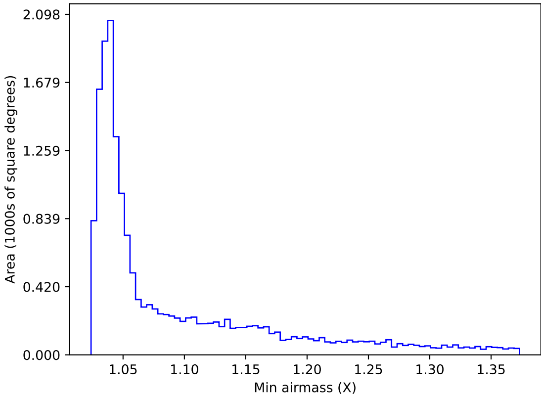
ddf_acor_sf10_lsf20_lsr20_v3.4_10yrs WFD u band: Min airmass
