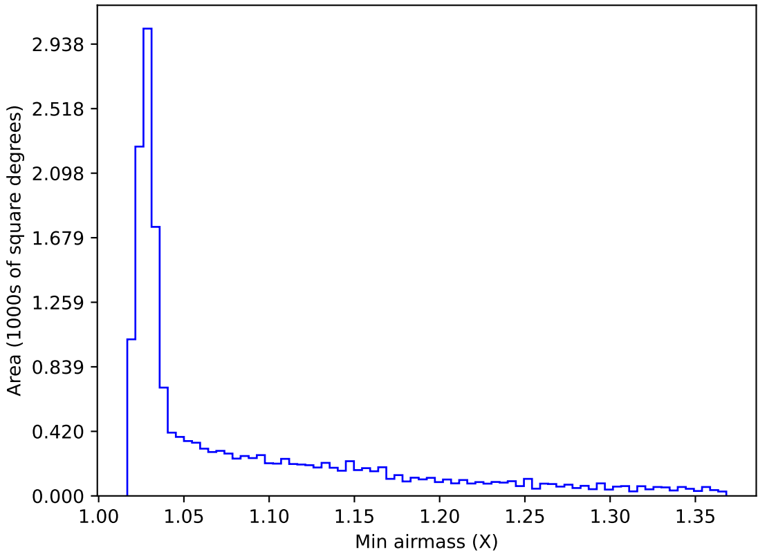
ddf_acor_sf10_lsf20_lsr20_v3.4_10yrs WFD r band: Min airmass
