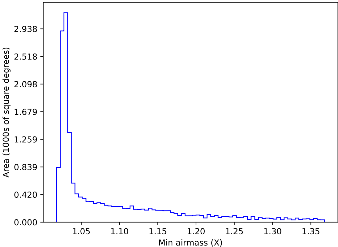
ddf_acor_sf10_lsf20_lsr20_v3.4_10yrs WFD i band: Min airmass
