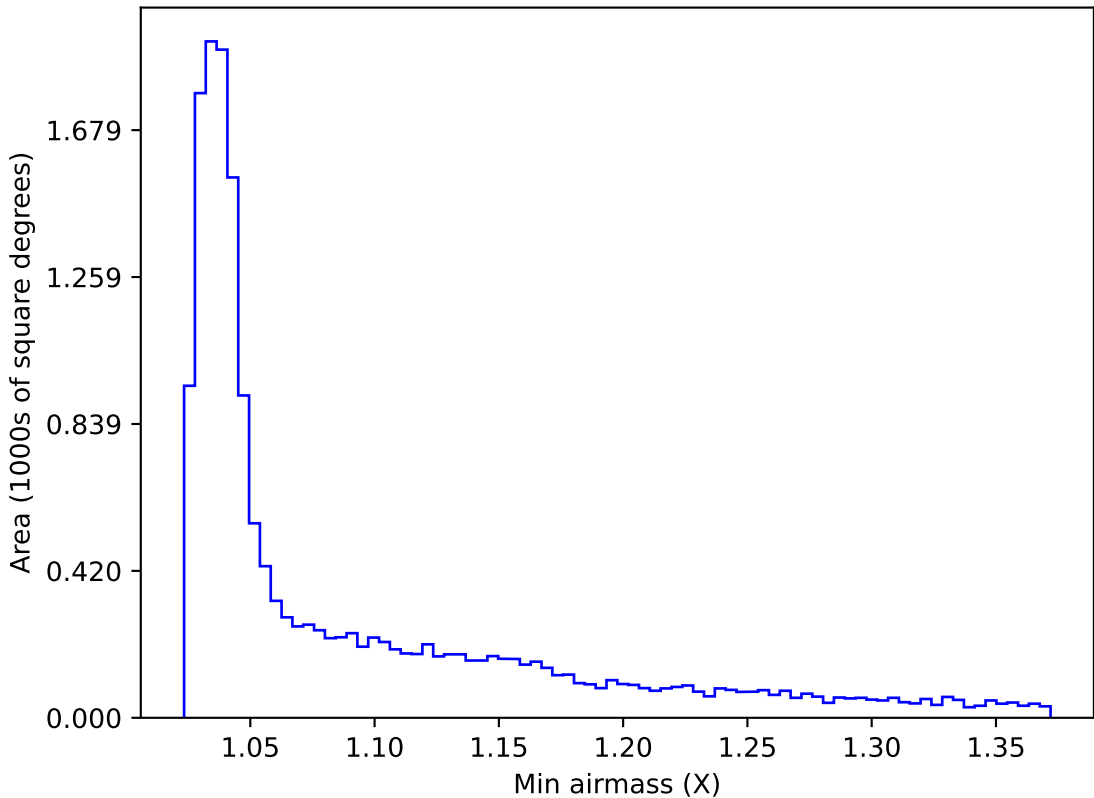
ddf_acor_sf10_lsf20_lsr20_v3.4_10yrs WFD g band: Min airmass
