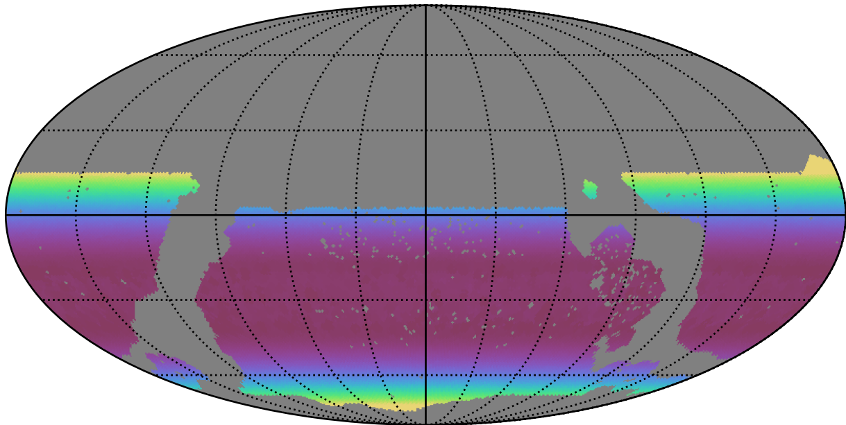
ddf_acor_sf10_lsf20_lsr20_v3.4_10yrs WFD all bands: Min airmass
