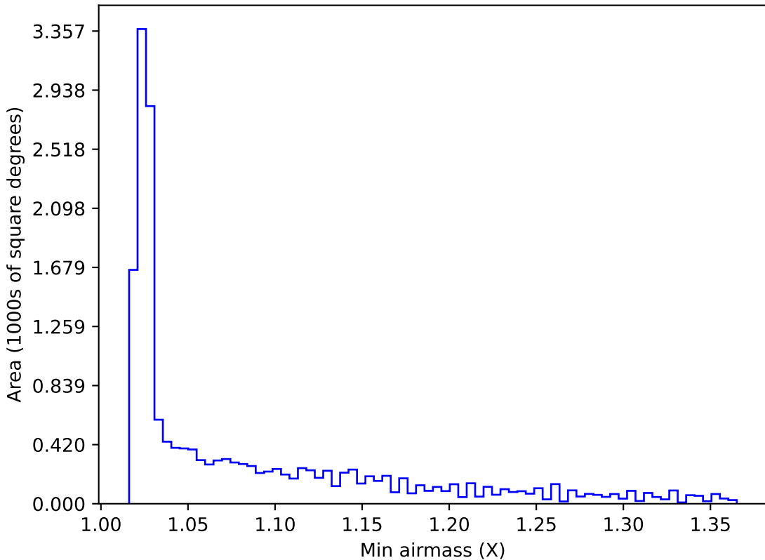
ddf_acor_sf10_lsf20_lsr20_v3.4_10yrs WFD all bands: Min airmass
