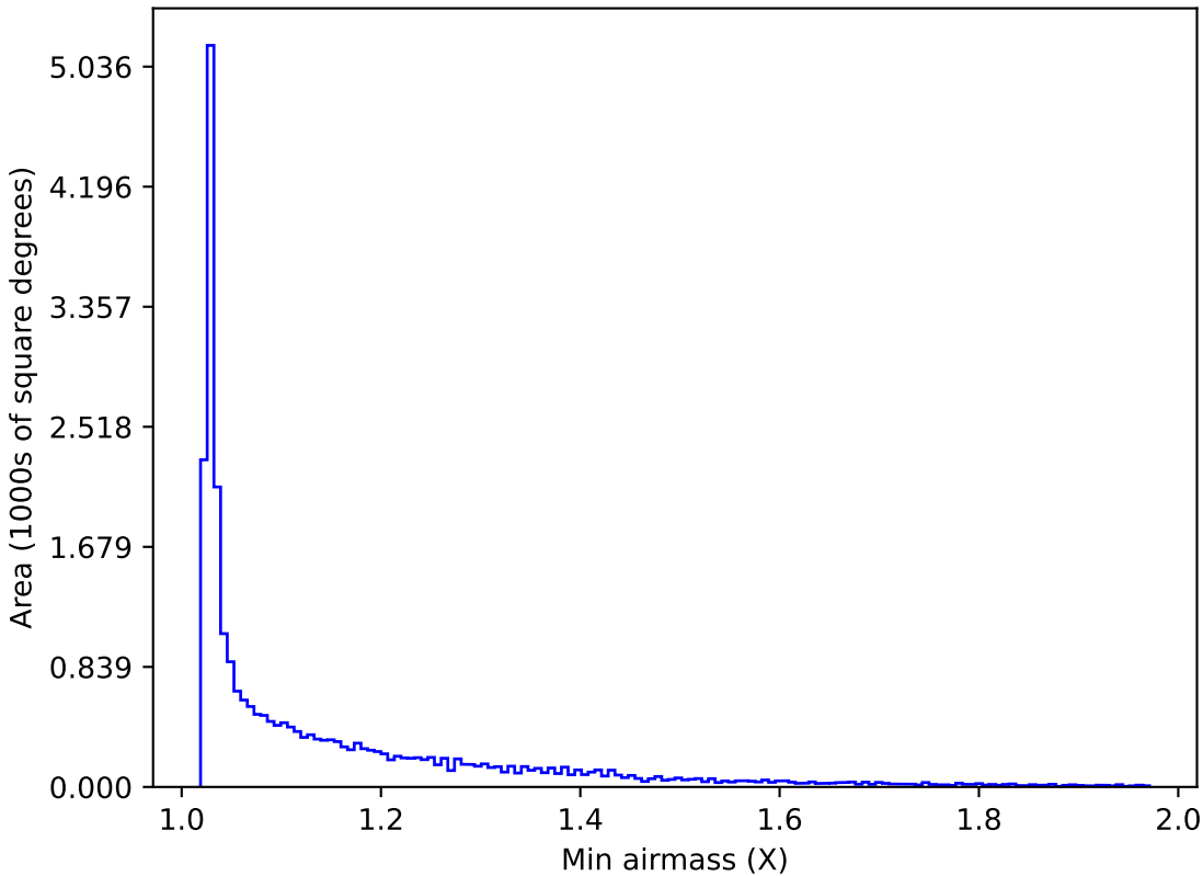
ddf_acor_sf10_lsf20_lsr20_v3.4_10yrs All sky z band: Min airmass
