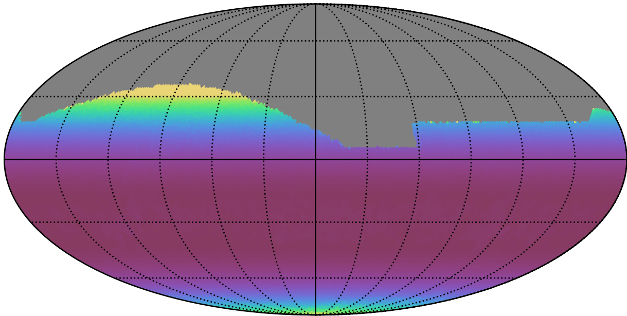
ddf_acor_sf10_lsf20_lsr20_v3.4_10yrs All sky r band: Min airmass
