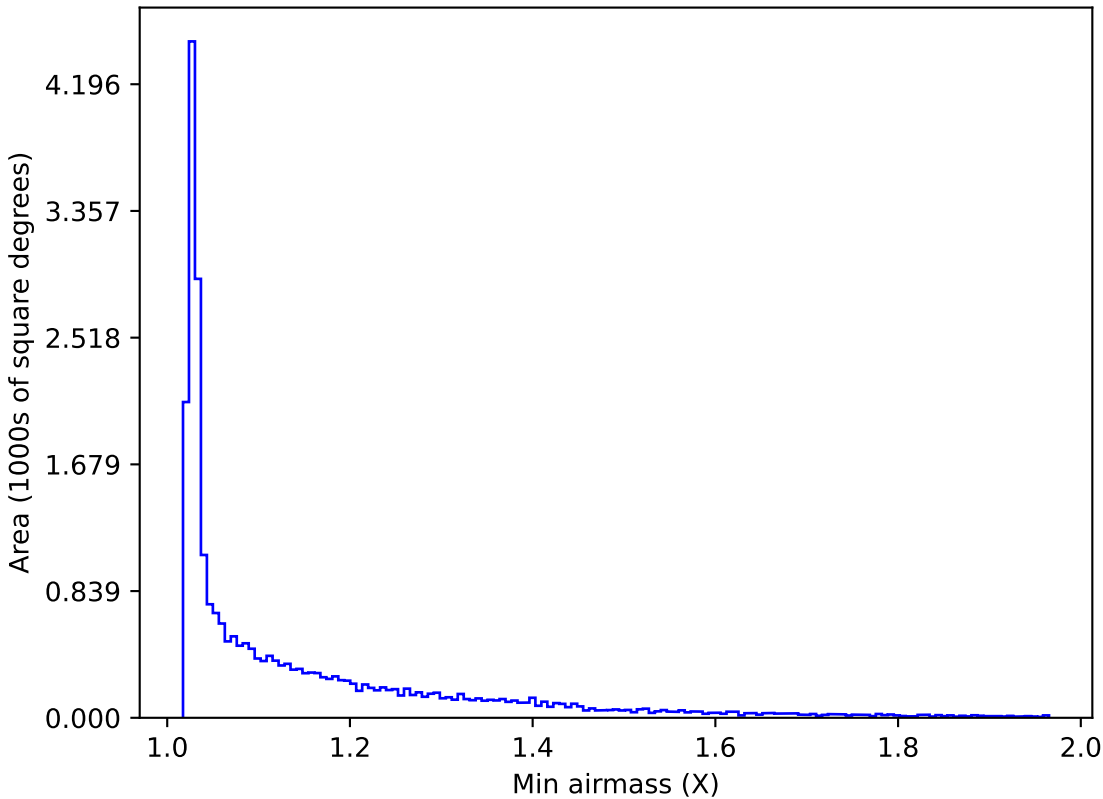
ddf_acor_sf10_lsf20_lsr20_v3.4_10yrs All sky r band: Min airmass
