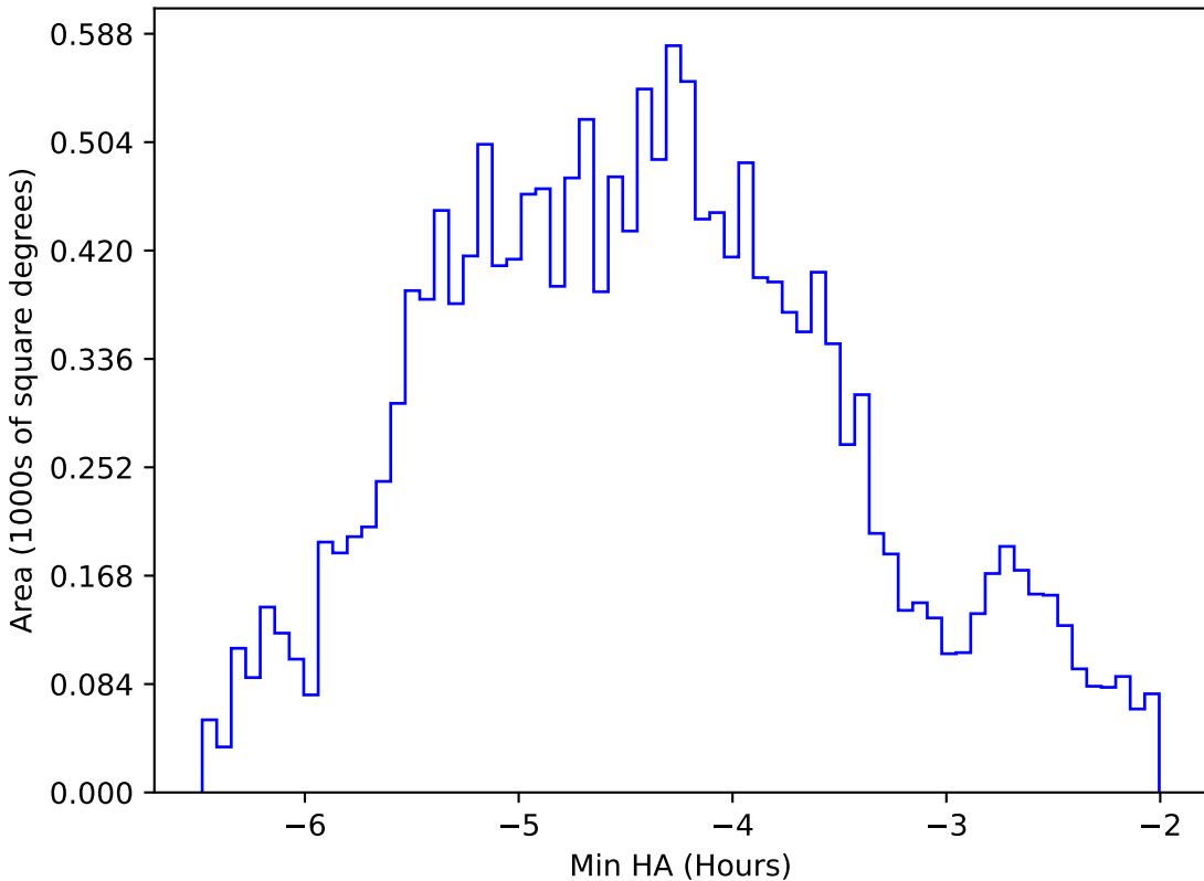
ddf_acor_sf10_lsf20_lsr20_v3.4_10yrs WFD z band: Min HA
