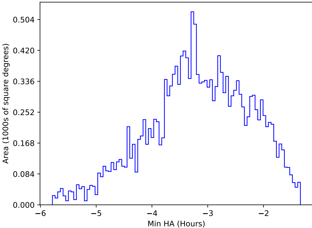
ddf_acor_sf10_lsf20_lsr20_v3.4_10yrs WFD u band: Min HA
