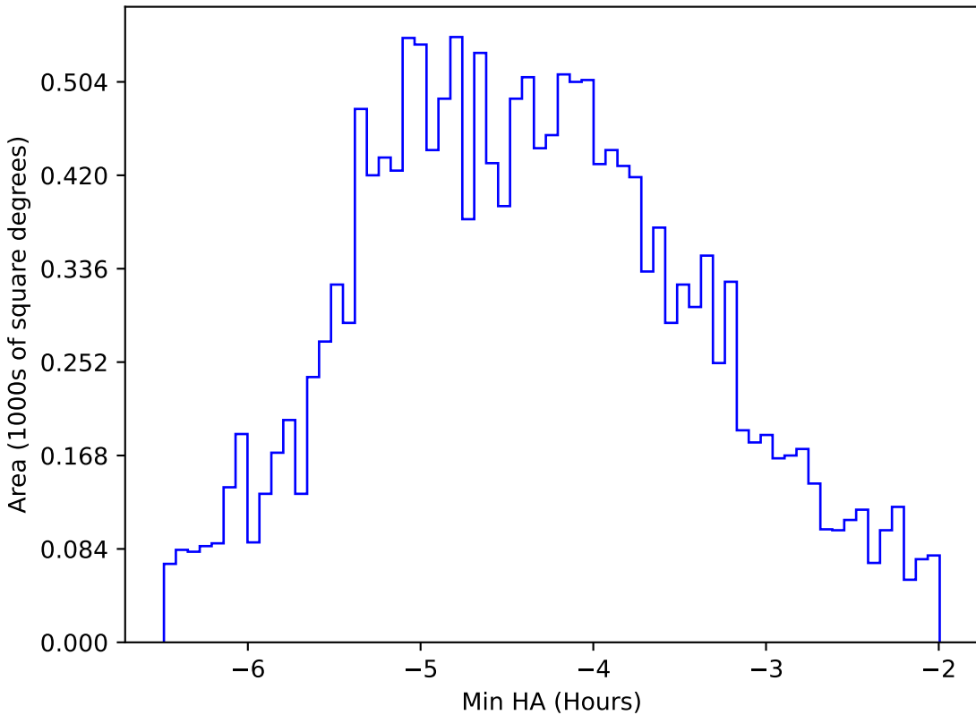
ddf_acor_sf10_lsf20_lsr20_v3.4_10yrs WFD i band: Min HA
