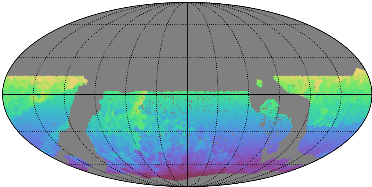
ddf_acor_sf10_lsf20_lsr20_v3.4_10yrs WFD all bands: Min HA
