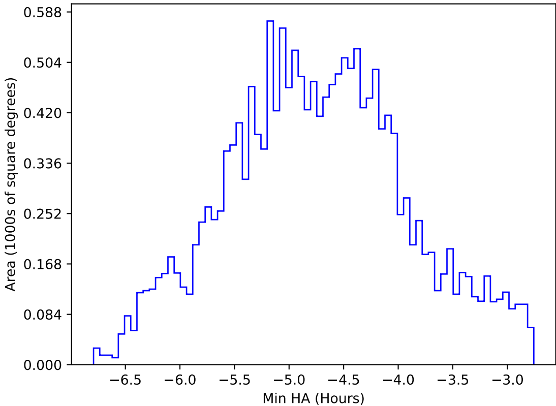
ddf_acor_sf10_ls20_lsr20_v3.4_10yrs WFD all bands: Min HA
