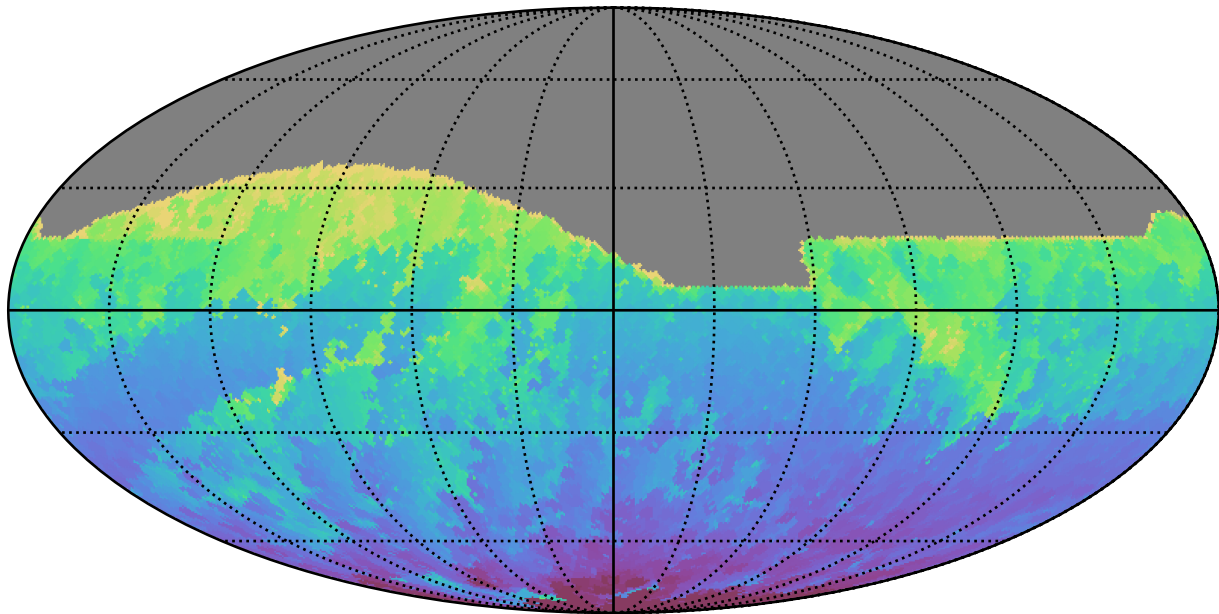
ddf_acor_sf10_lsf20_lsr20_v3.4_10yrs All sky z band: Min HA
