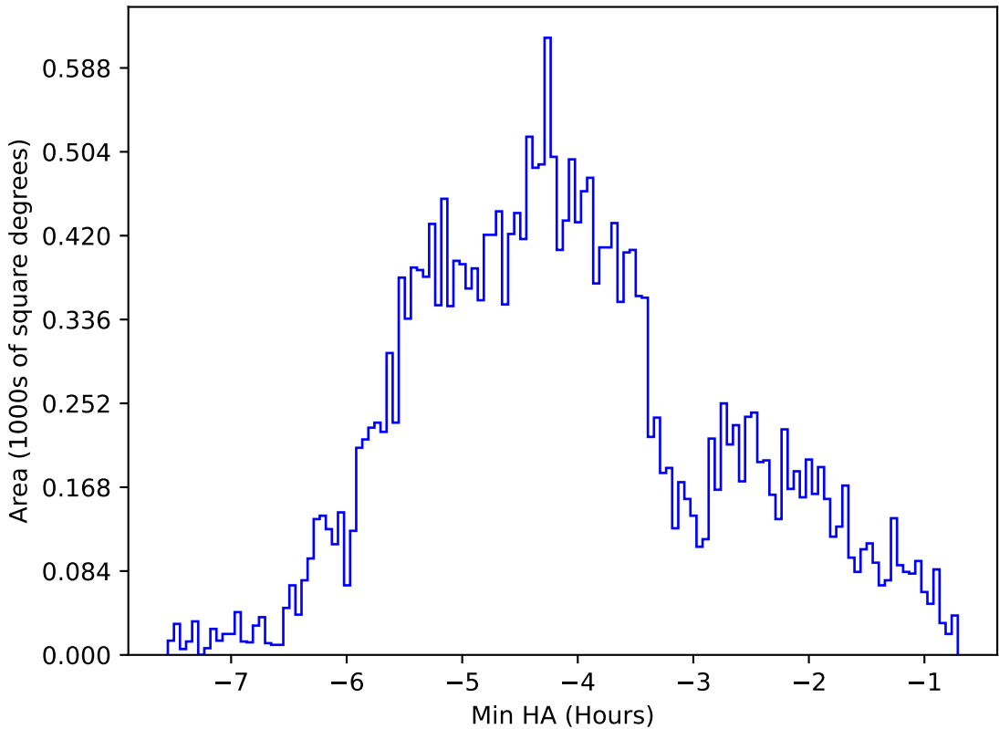
ddf_acor_sf10_lsf20_lsr20_v3.4_10yrs All sky z band: Min HA
