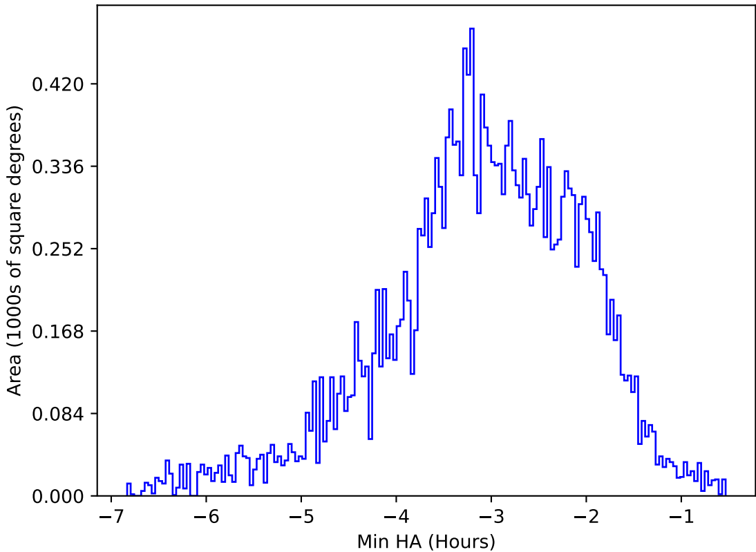
ddf_acor_sf10_lsf20_lsr20_v3.4_10yrs All sky u band: Min HA
