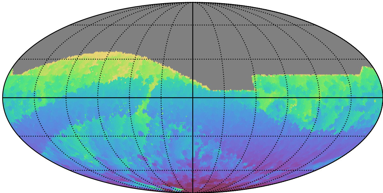
ddf_acor_sf10_lsf20_lsr20_v3.4_10yrs All sky r band: Min HA
