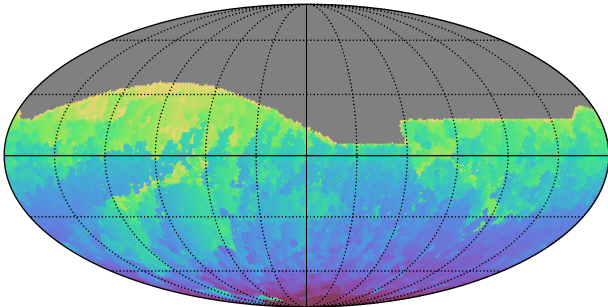
ddf_acor_sf10_lsf20_lsr20_v3.4_10yrs All sky i band: Min HA
