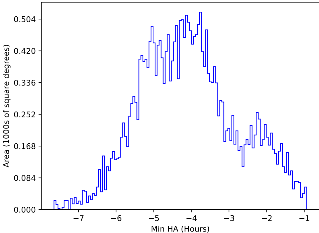
ddf_acor_sf10_ls20_lsr20_v3.4_10yrs All sky i band: Min HA
