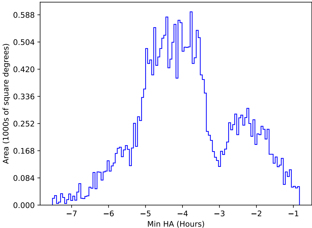
ddf_acor_sf10_lsf20_lsr20_v3.4_10yrs All sky g band: Min HA
