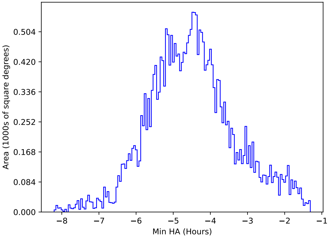
ddf_acor_sf10_lsf20_lsr20_v3.4_10yrs All sky all bands: Min HA
