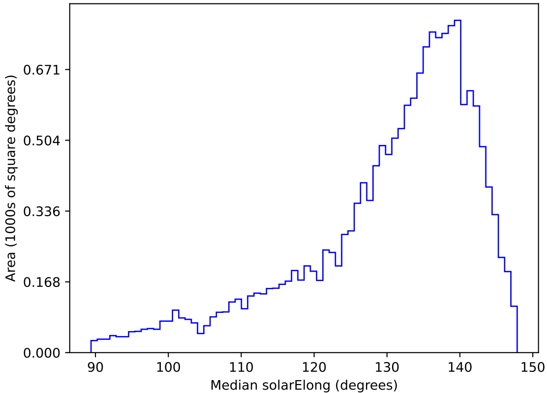
ddf_acor_sf10_lsf20_lsr20_v3.4_10yrs WFD y band: Median solarElong
