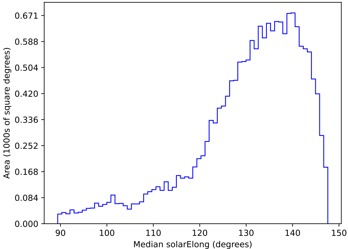
ddf_acor_sf10_lsf20_lsr20_v3.4_10yrs WFD r band: Median solarElong
