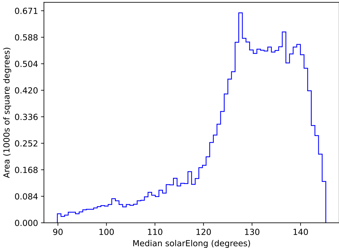
ddf_acor_sf10_lsf20_lsr20_v3.4_10yrs WFD i band: Median solarElong
