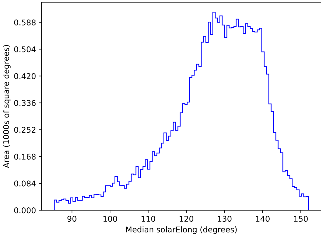
ddf_acor_sf10_lsf20_lsr20_v3.4_10yrs All sky z band: Median solarElong
