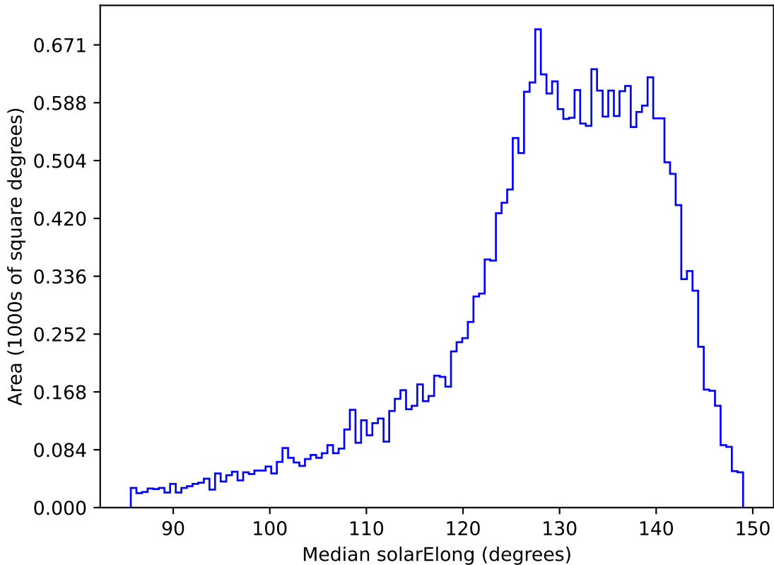
ddf_acor_sf10_lsf20_lsr20_v3.4_10yrs All sky i band: Median solarElong
