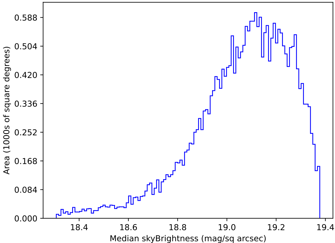
ddf_acor_sf10_lsf20_lsr20_v3.4_10yrs Yr 1 z band: Median skyBrightness
