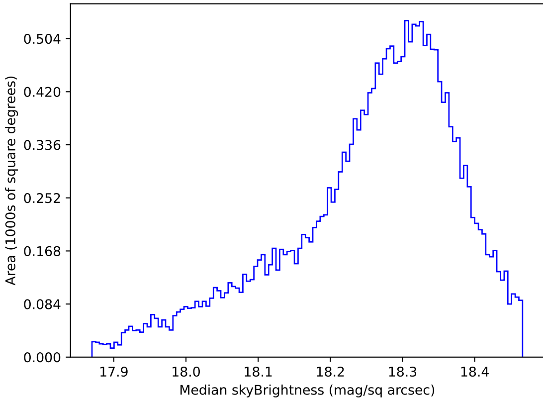
ddf_acor_sf10_lsf20_lsr20_v3.4_10yrs Yr 1 y band: Median skyBrightness
