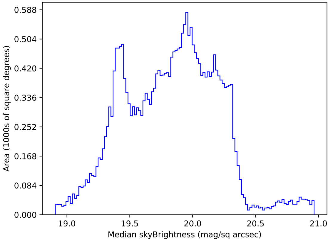
ddf_acor_sf10_lsf20_lsr20_v3.4_10yrs Yr 1 all bands: Median skyBrightness
