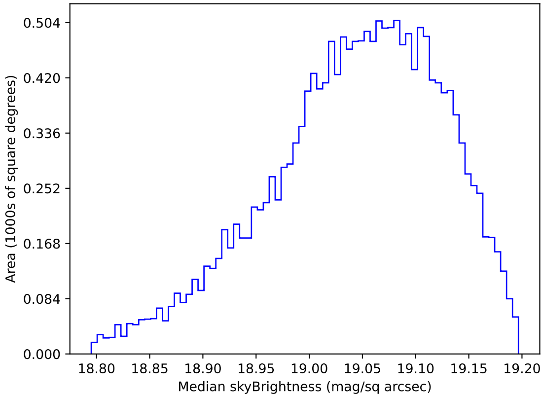
ddf_acor_sf10_lsf20_lsr20_v3.4_10yrs WFD z band: Median skyBrightness
