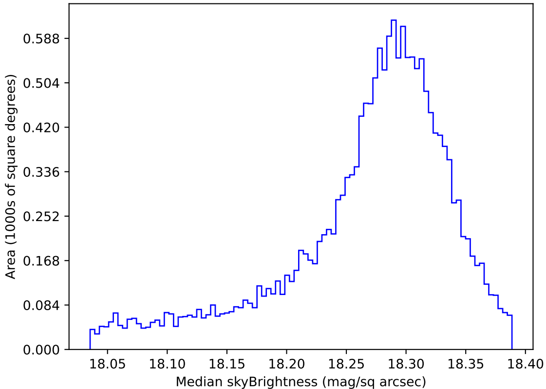
ddf_acor_sf10_lsf20_lsr20_v3.4_10yrs WFD y band: Median skyBrightness
