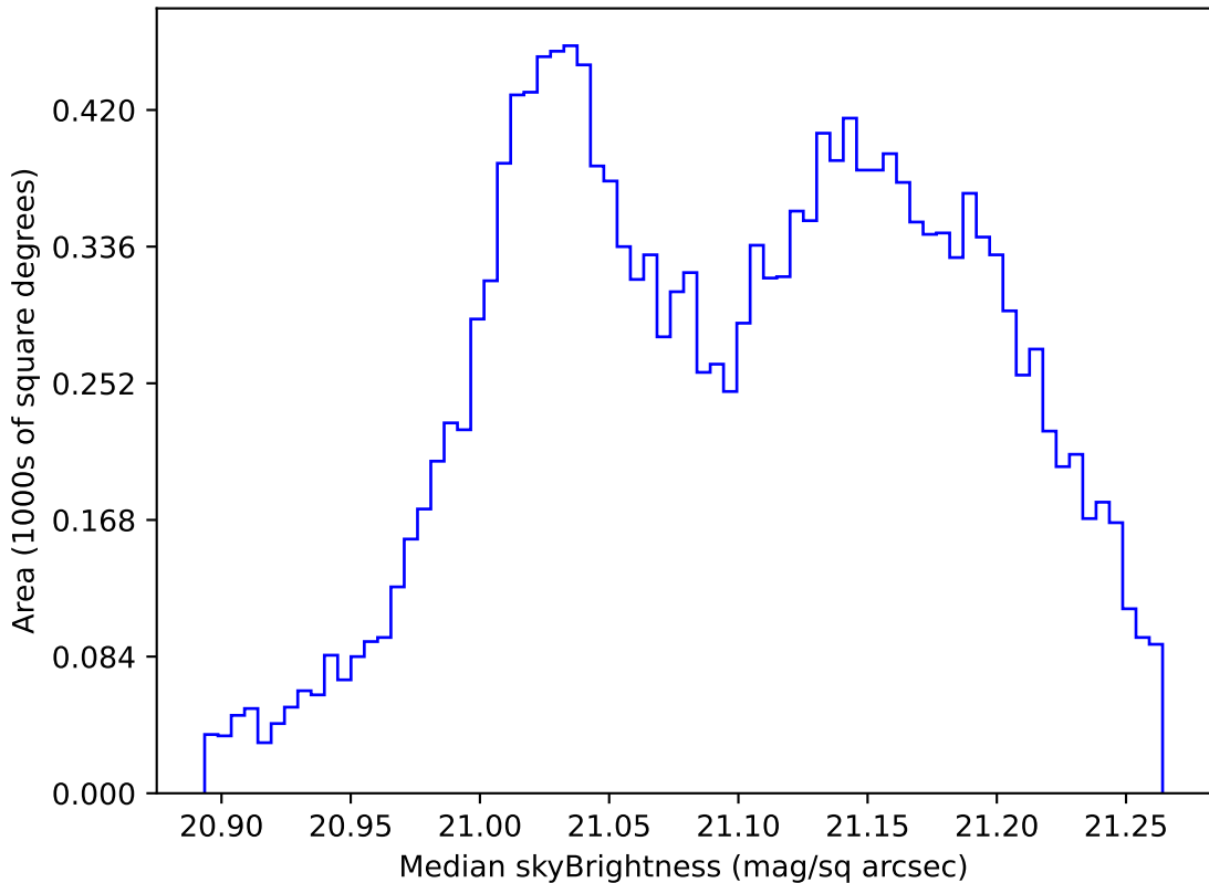
ddf_acor_sf10_lsf20_lsr20_v3.4_10yrs WFD r band: Median skyBrightness
