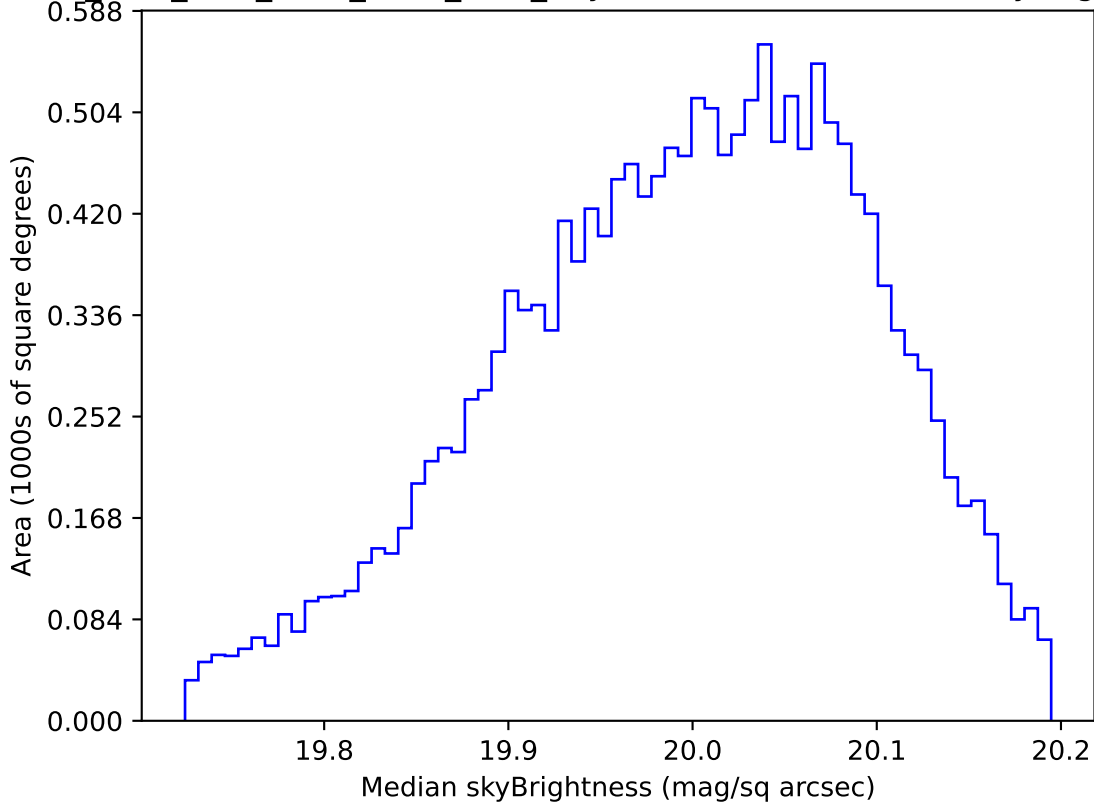
ddf_acor_sf10_lsf20_lsr20_v3.4_10yrs WFD i band: Median skyBrightness
