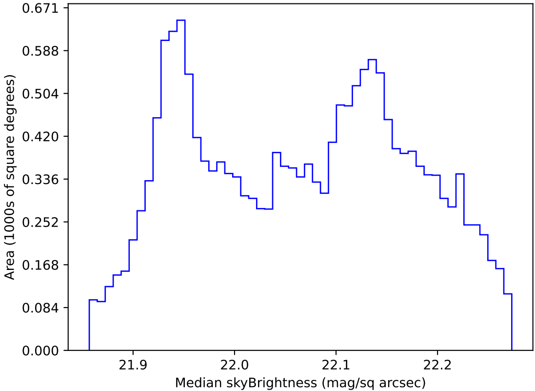
ddf_acor_sf10_lsf20_lsr20_v3.4_10yrs WFD g band: Median skyBrightness
