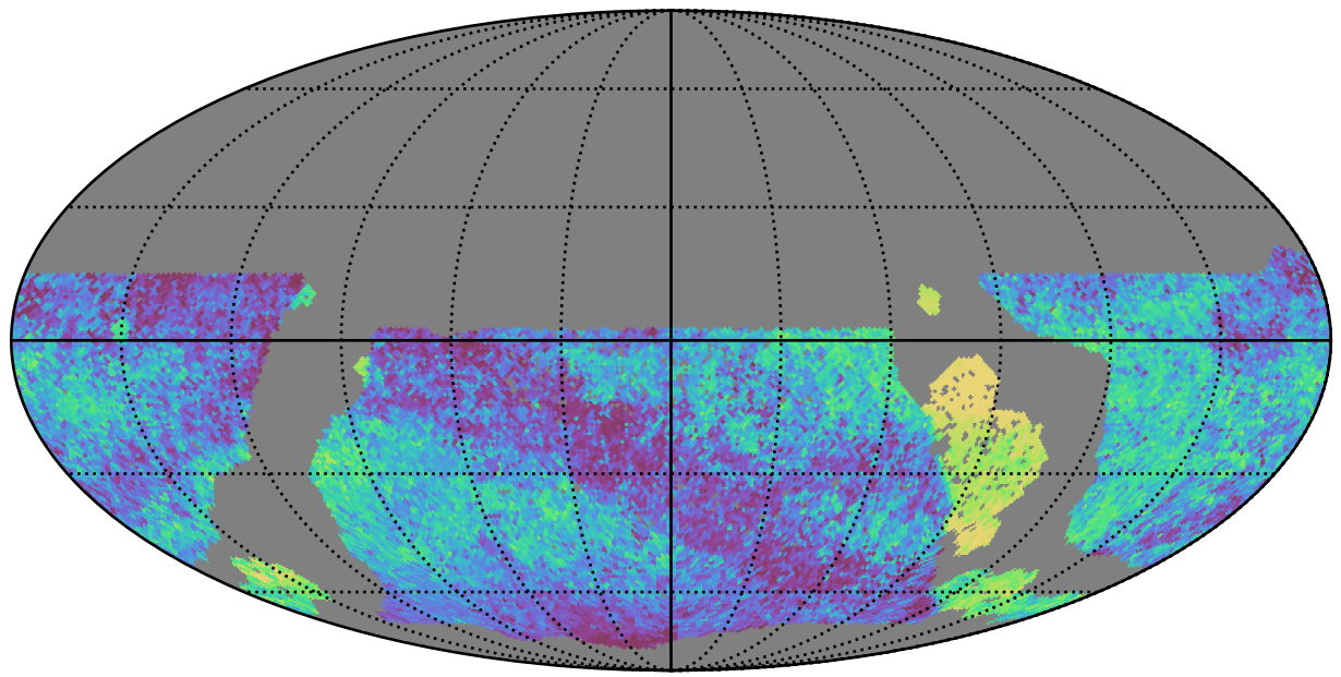
ddf_acor_sf10_lsf20_lsr20_v3.4_10yrs WFD all bands: Median skyBrightness
