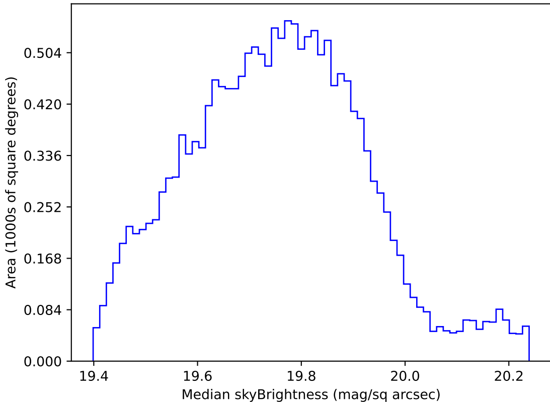
ddf_acor_sf10_lsf20_lsr20_v3.4_10yrs WFD all bands: Median skyBrightness
