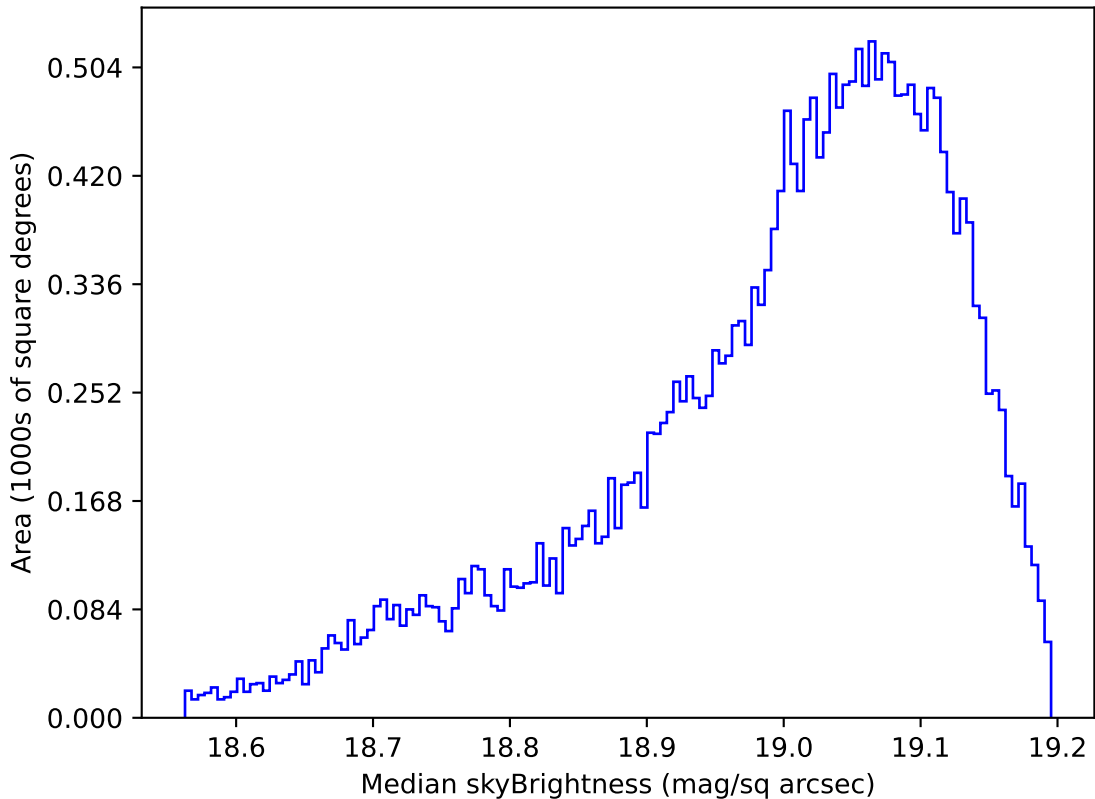
ddf_acor_sf10_lsf20_lsr20_v3.4_10yrs All sky z band: Median skyBrightness
