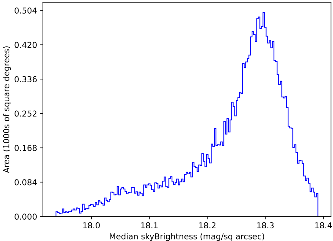
ddf_acor_sf10_lsf20_lsr20_v3.4_10yrs All sky y band: Median skyBrightness
