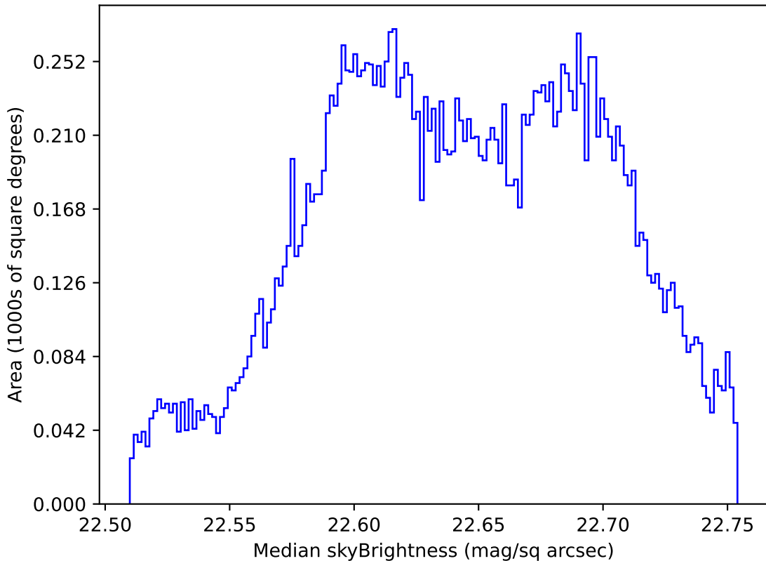
ddf_acor_sf10_lsf20_lsr20_v3.4_10yrs All sky u band: Median skyBrightness
