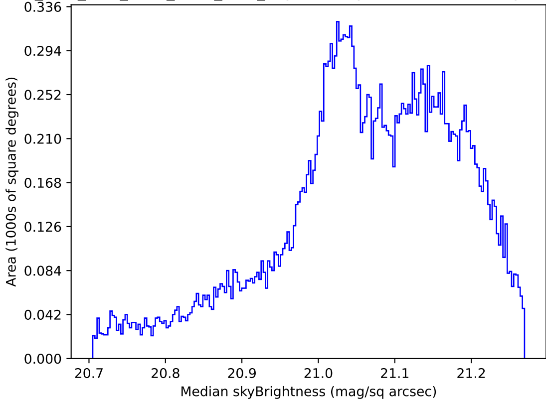
ddf_acor_sf10_lsf20_lsr20_v3.4_10yrs All sky r band: Median skyBrightness
