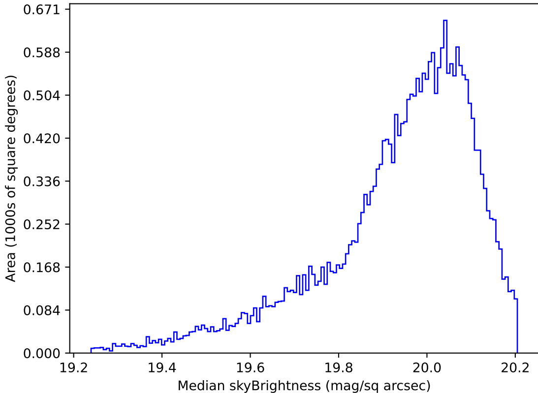
ddf_acor_sf10_lsf20_lsr20_v3.4_10yrs All sky i band: Median skyBrightness
