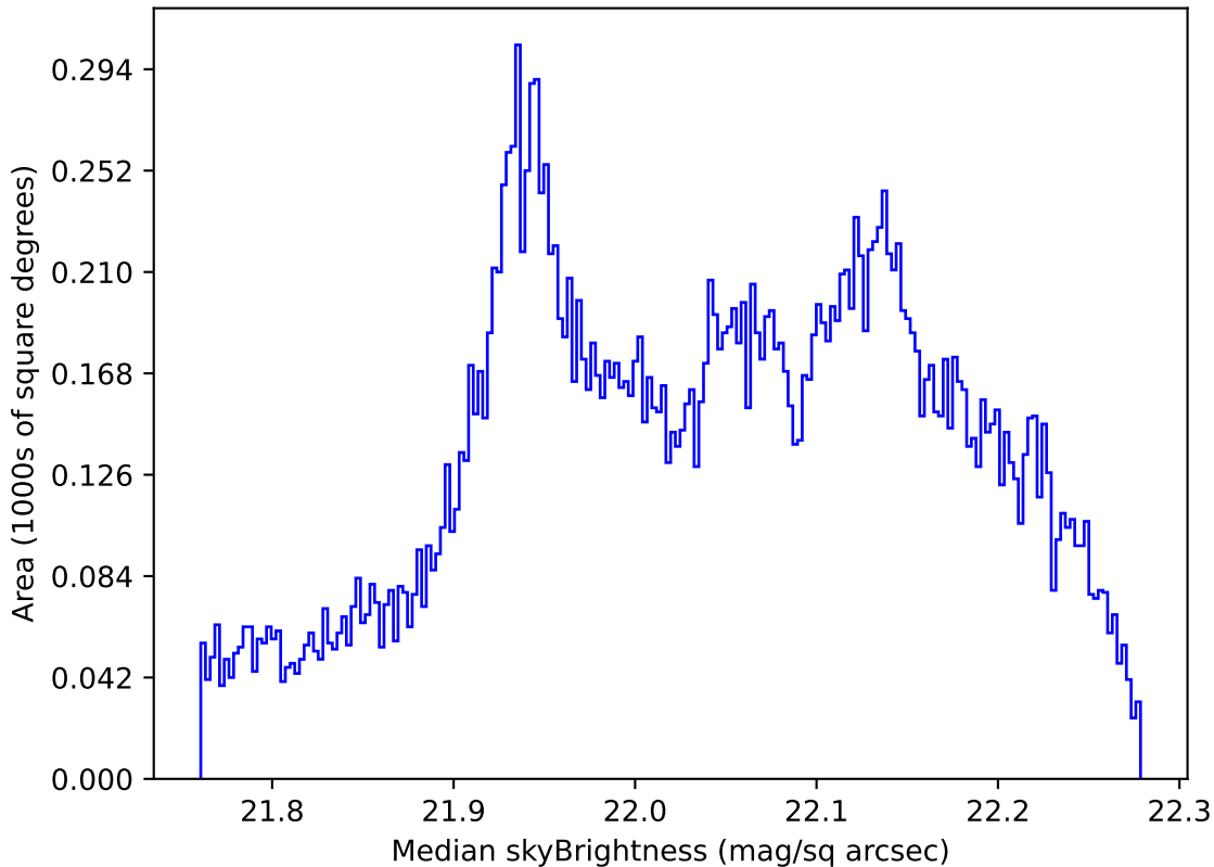
ddf_acor_sf10_lsf20_lsr20_v3.4_10yrs All sky g band: Median skyBrightness
