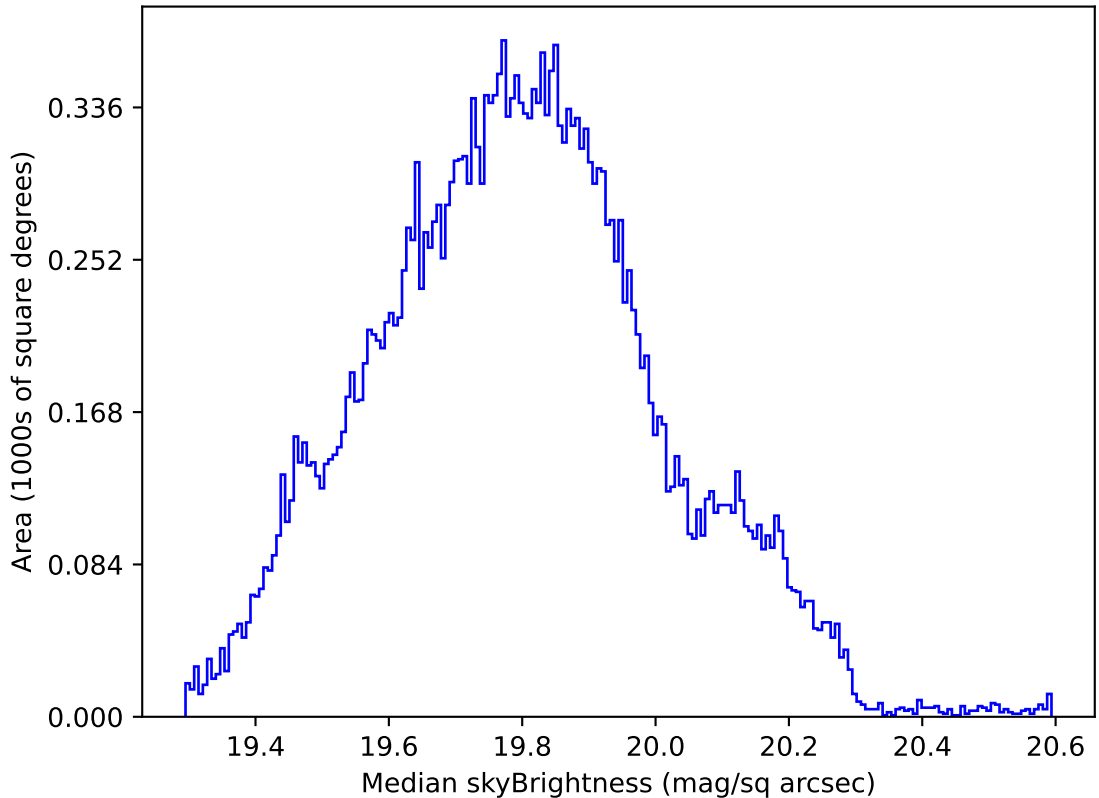
ddf_acor_sf10_lsf20_lsr20_v3.4_10yrs All sky all bands: Median skyBrightness
