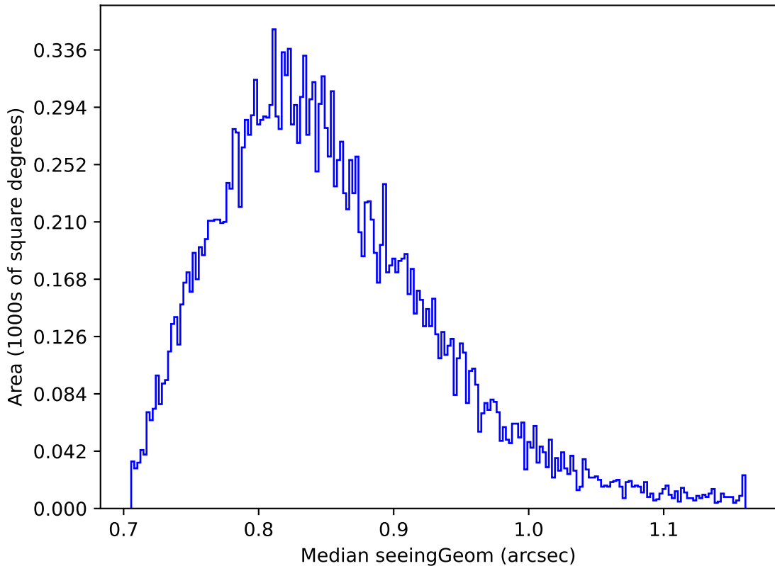
ddf_acor_sf10_lsf20_lsr20_v3.4_10yrs Yr 1 y band: Median seeingGeom
