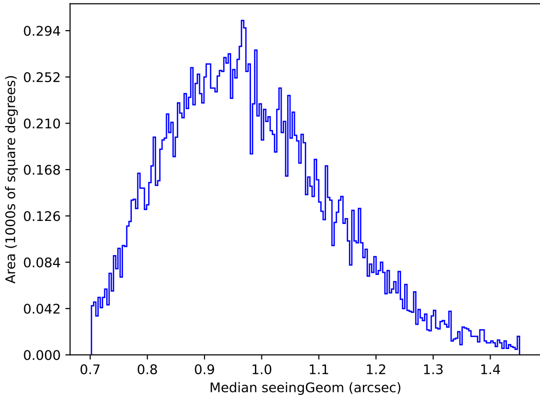
ddf_acor_sf10_lsf20_lsr20_v3.4_10yrs Yr 1 u band: Median seeingGeom
