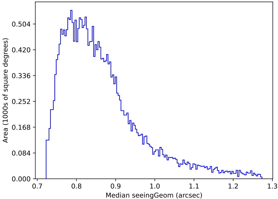
ddf_acor_sf10_lsf20_lsr20_v3.4_10yrs Yr 1 all bands: Median seeingGeom
